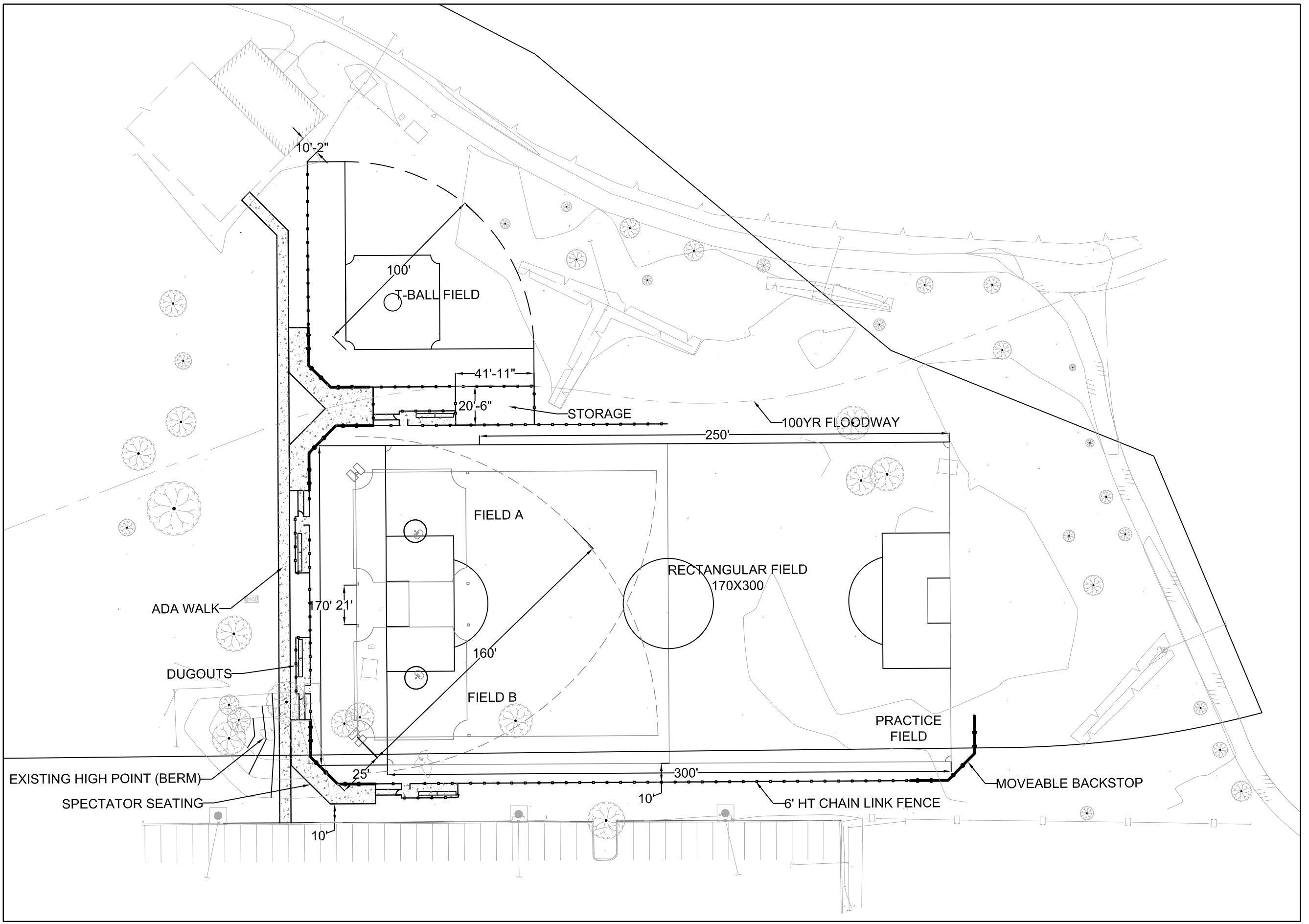
A1 FIELD LAYOUT OPTION A
