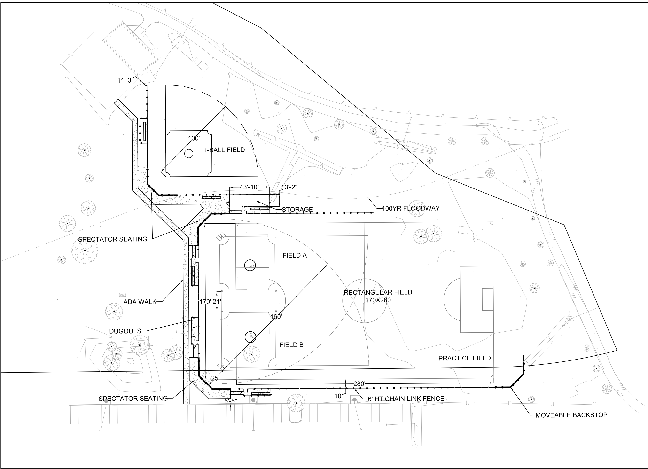
A3 FIELD LAYOUT OPTION C
