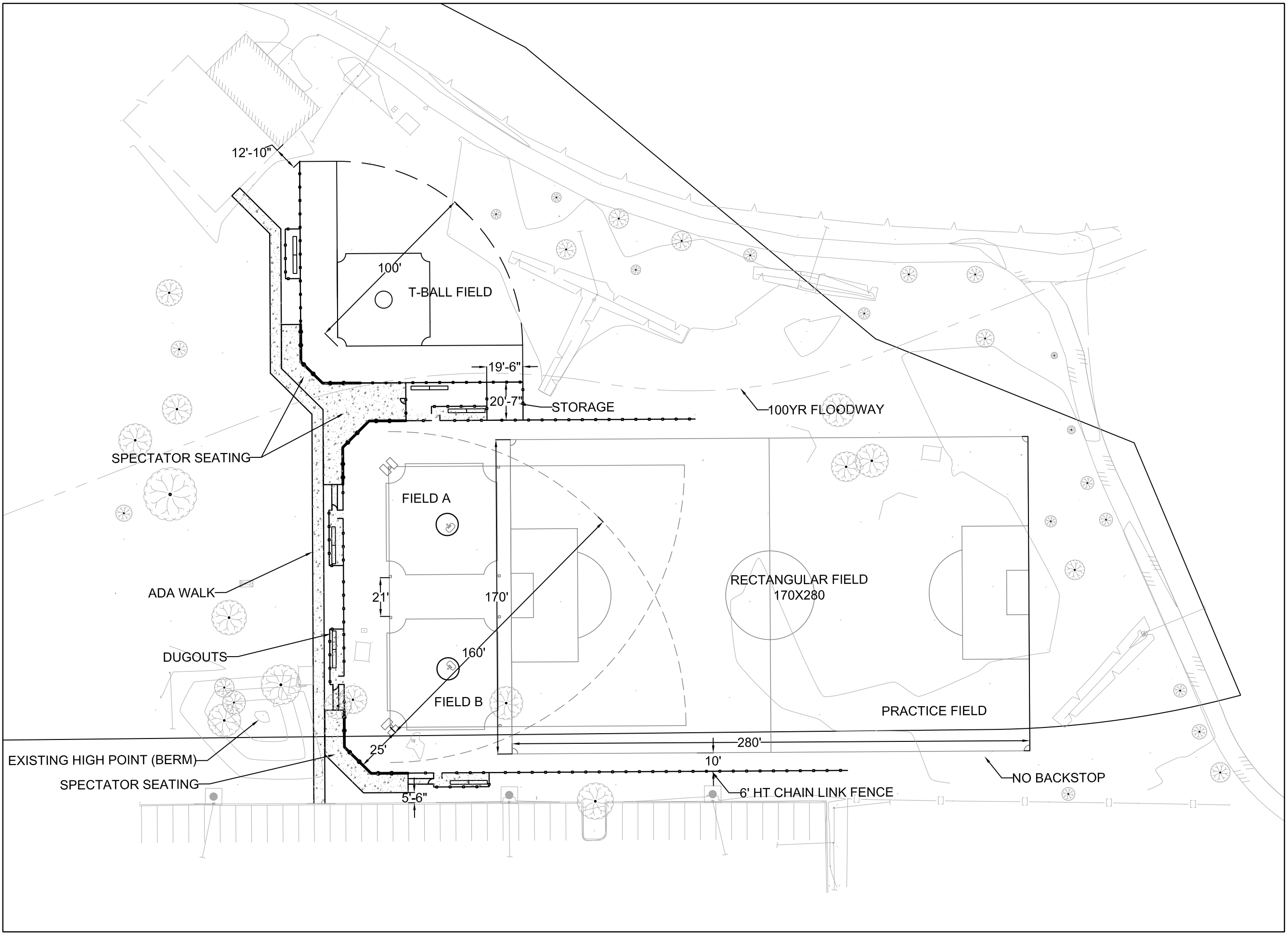
A2 FIELD LAYOUT OPTION B
